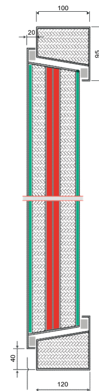
CORTE VERTICAL
